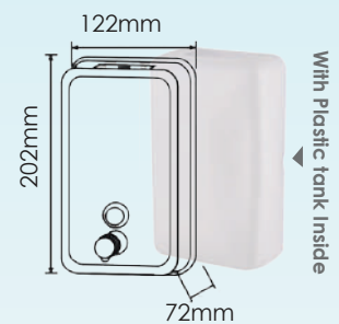
ELSD 1200BLD SOAP DISPENSER (Manual) SS 304GRADE Satin Finish
