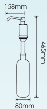
ELFSD 1000P FOAMING SOAP DISPENSER ( Counter Top)
