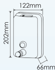
ELSD 1000A SOAP DISPENSER (Manual) SS 304GRADE Mirror Finish
