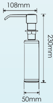
ELSSD 250SS SOAP DISPENSER (Counter Top)
